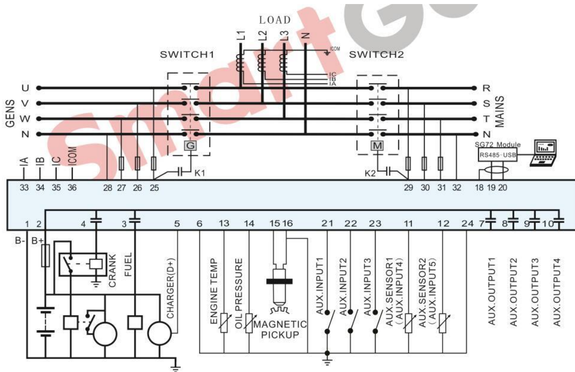
HGM4020NC Typical Application
